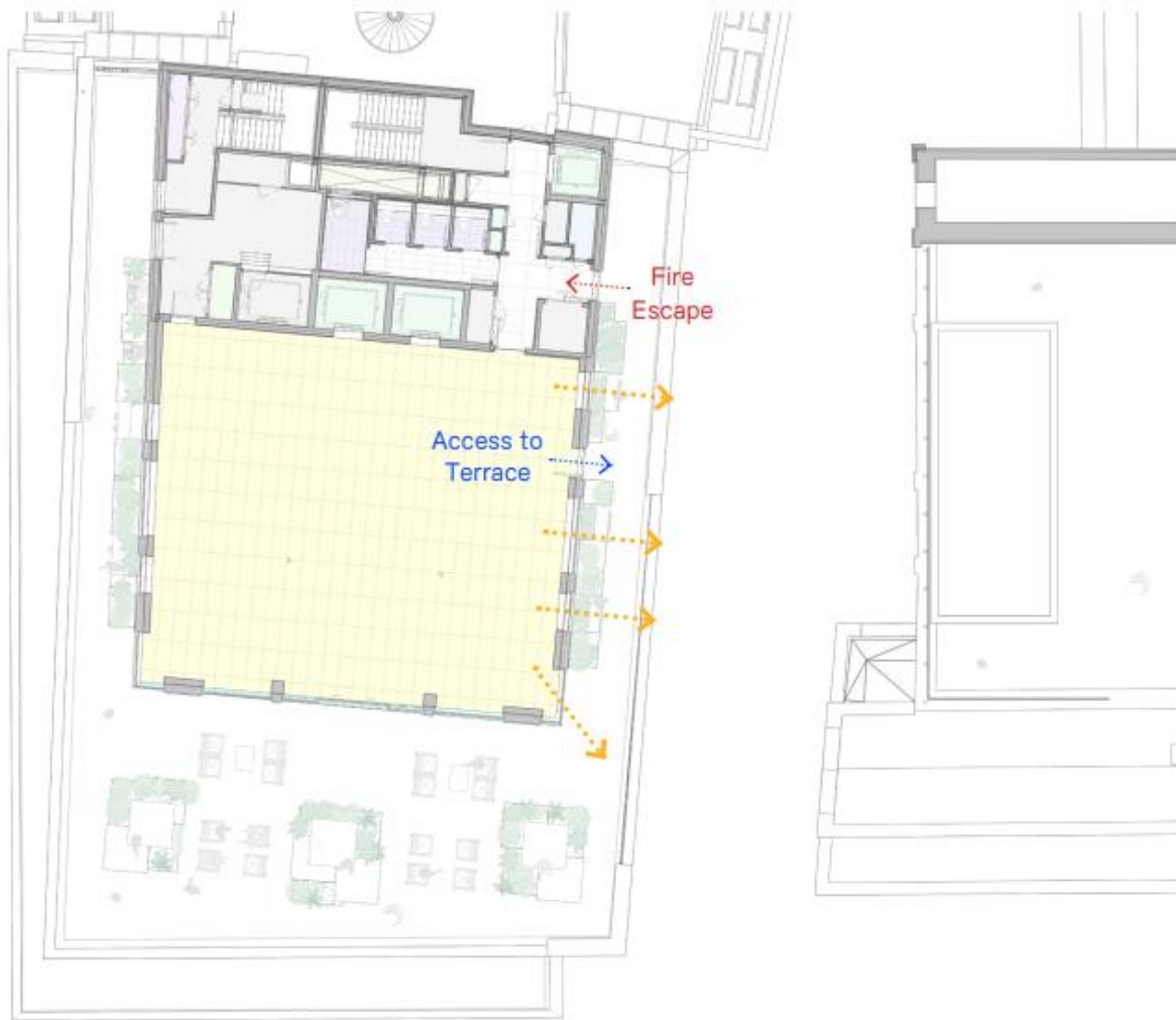
Initial Proposed Roof terrace and Pavilion layout
